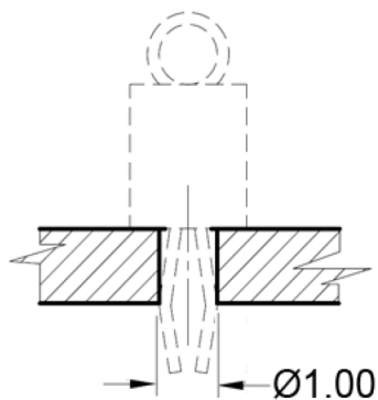
(MOUNTING DETAIL)
